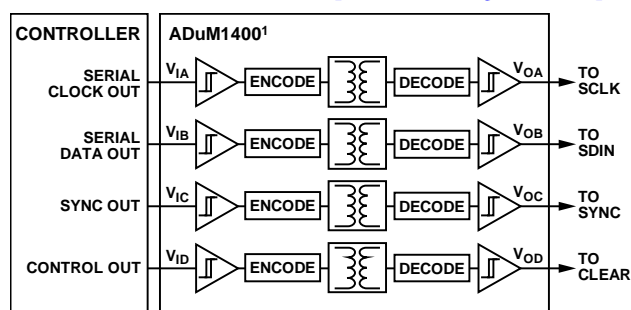
Figure 57. Isolated Interface
