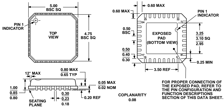
COMPLIANT TO JEDEC STANDARDS MO-220-VHDD-2 Figure 58. 32-Lead Lead Frame Chip Scale Package [LFCSP_VQ] 5 mm × 5 mm Body, Very Thin Quad (CP-32-2) Dimensions shown in millimeters
