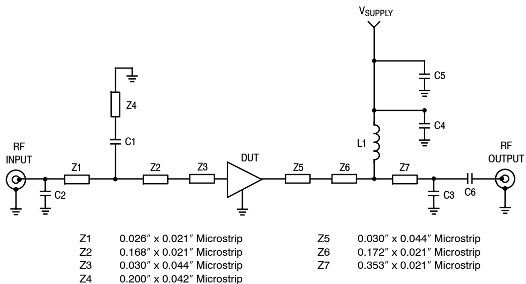
Figure 4. MMG15241HT1 Test Circuit Schematic
