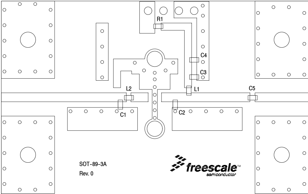
Figure 14. MMG15241HT1 Test Circuit Component Layout
