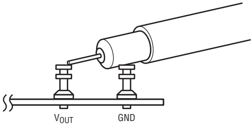
Figure 4. Measuring Input or Output Ripple
