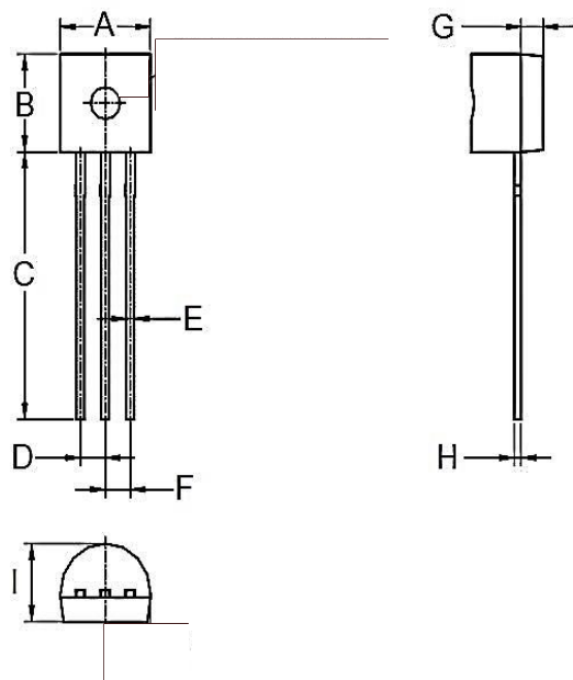
TO-92 Bulk
