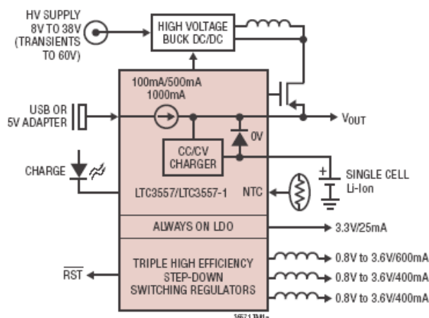
Figure 1. LTC3557/LTC3557-1 Simplified Typical Application
