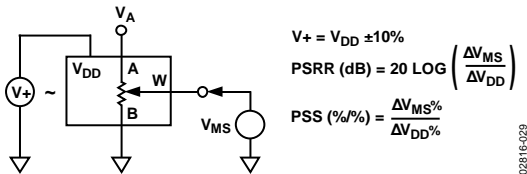
Figure 30. Power Supply Sensitivity (PSS, PSRR)
