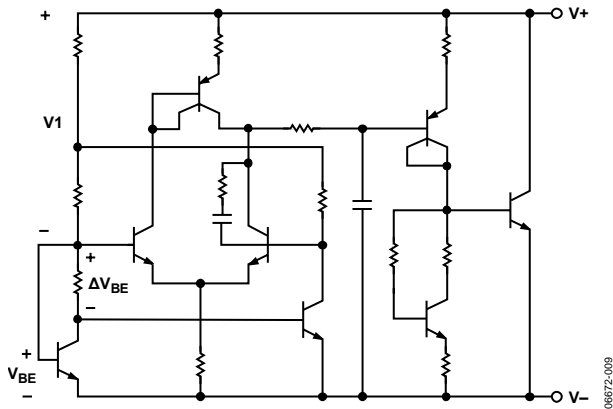
Figure 9. Schematic Diagram
