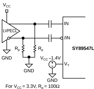
Figure 4d. LVPECL Interface (AC-Coupled)
