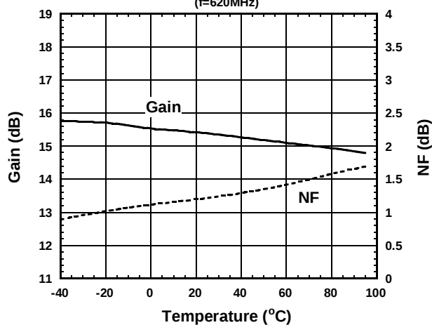
Gain, NF vs. Temperature
