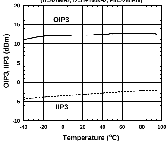
OIP3, IIP3 vs. Temperature
