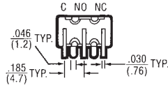
1 Pole P.C. Mounting
