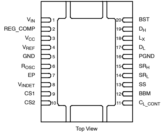
Si9122DLP (MLP65-20)
