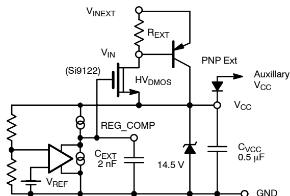
Figure 5. High-Voltage Pre-Regulator Circuit
