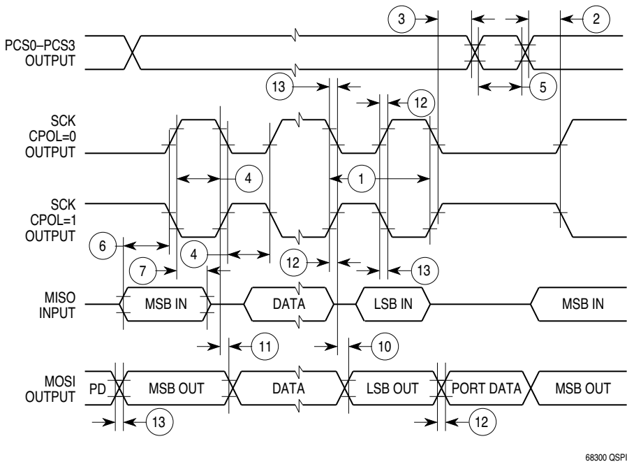
Figure A-16 QSPI Timing — Master, CPHA = 0
