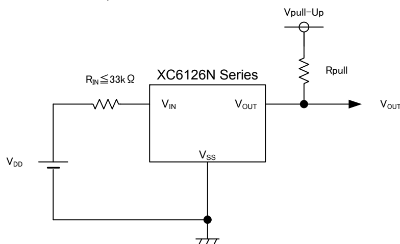
[Figure 1: Circuit connected with the input resistor for N-ch open drain]
