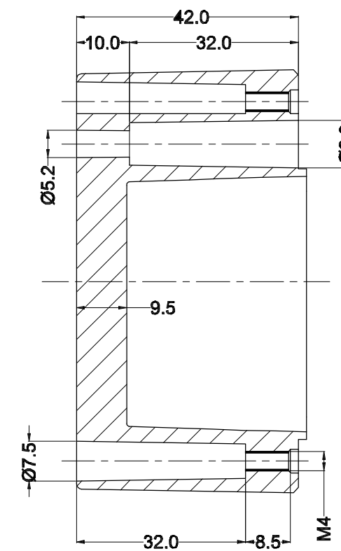
SECTION B-B
