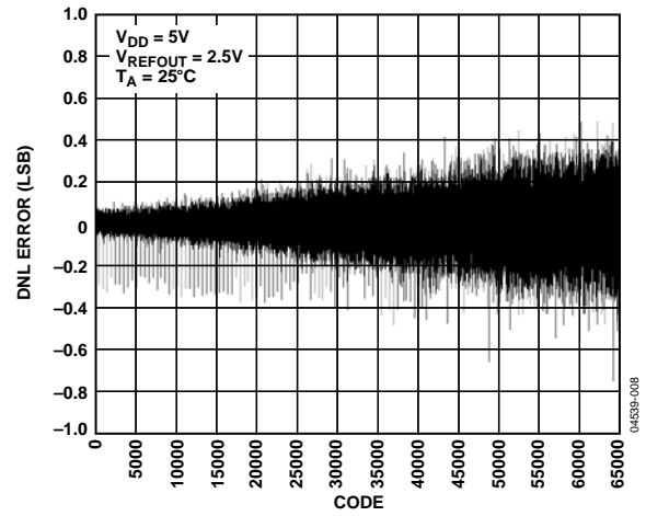
Figure 9. DNL—AD5660-2/AD5660-3
