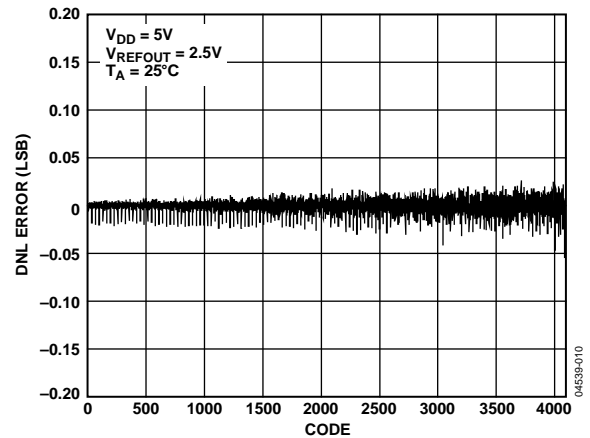
Figure 11. DNL—AD5620-2/AD6520-3
