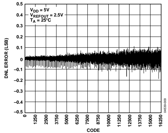
Figure 10. DNL—AD5640-2/AD5640-3
