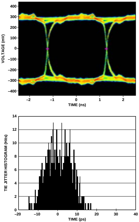
Figure 65. Data Eye for LVDS Outputs in ANSI-644 Mode with 6-Inch Trace Lengths on Standard FR-4, AD9467-250
