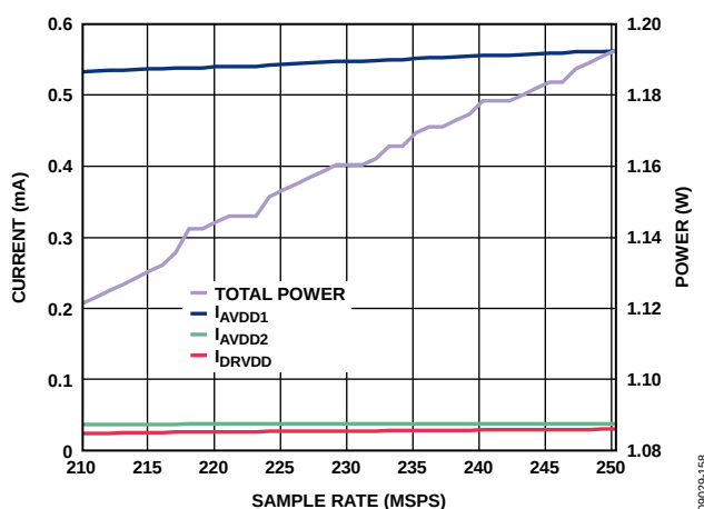
Figure 63. Supply Current vs. f_{\text{SAMPLE}} for f_{\text{IN}} = 5 MHz, AD9467-250
