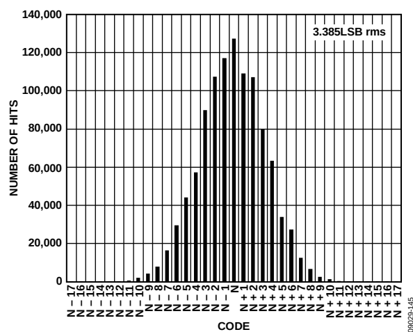
Figure 45. Input-Referred Noise Histogram, 2.5 V p-p FS, AD9467-250
