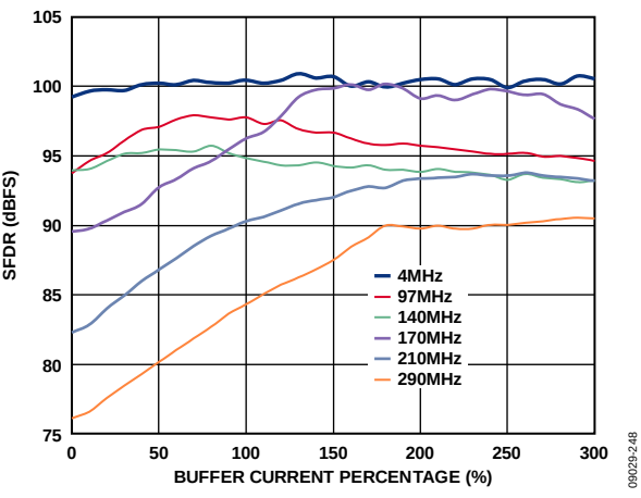
Figure 48. SFDR Performance vs. Buffer Current Percentage Over Analog Input Frequency, AD9467-250
