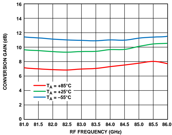
Figure 70. Conversion Gain vs. RF Frequency at Various Temperatures, RFIN = -20 dBm, LO = 2 dBm, IF = 2000 MHz, VDLNA = 4 V
