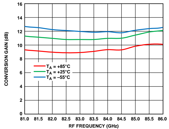
Figure 73. Conversion Gain vs. RF Frequency at Various Temperatures, RFIN = -20 dBm, LO = 2 dBm, IF = 2000 MHz, VDLNA = 3 V
