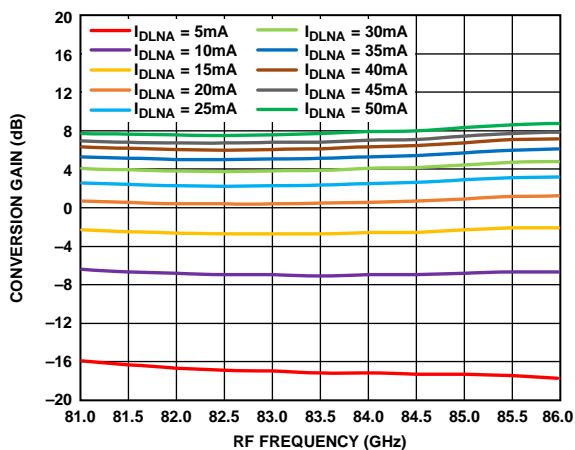
Figure 72. Conversion Gain vs. RF Frequency at Various IDLNA Values, RFIN = -20 dBm, LO = 2 dBm, IF = 2000 MHz, VDLNA = 4 V
