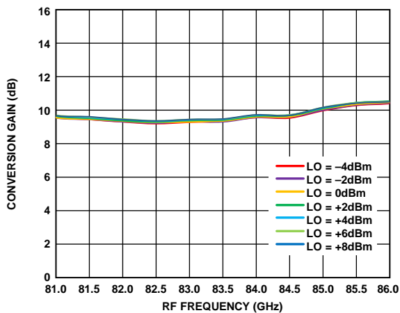
Figure 71. Conversion Gain vs. RF Frequency at Various LO Powers, RFIN = -20 dBm, IF = 2000 MHz, VDLNA = 4 V
