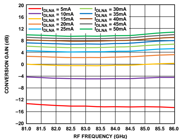
Figure 75. Conversion Gain vs. RF Frequency at Various IDLNA Values, RFIN = -20 dBm, LO = 2 dBm, IF = 2000 MHz, VDLNA = 3 V
