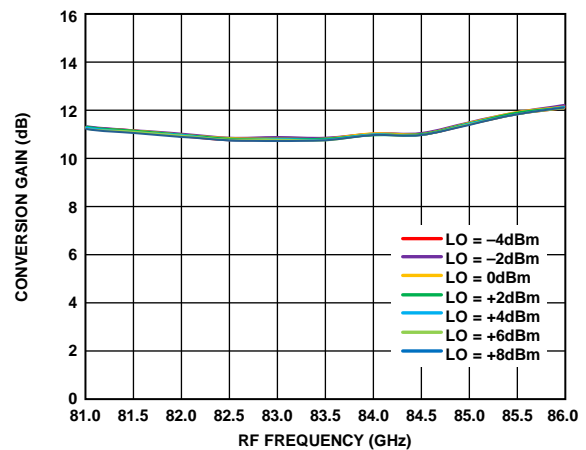
Figure 74. Conversion Gain vs. RF Frequency at Various LO Powers, RFIN = -20 dBm, IF = 2000 MHz, VDLNA = 3 V
