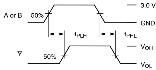
Figure 4. Switching Waveforms
