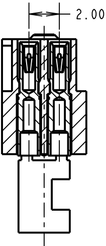
SECTION X-X
