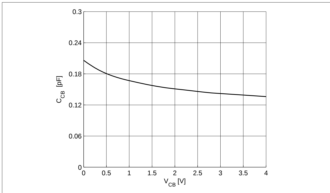
Figure 5-12 Collector Base Capacitance C_{CB} = f(V_{CB}) , f = 1 MHz
