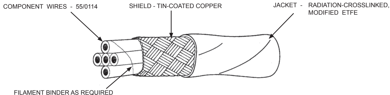
CABLE CONSTRUCTION DETAILS
