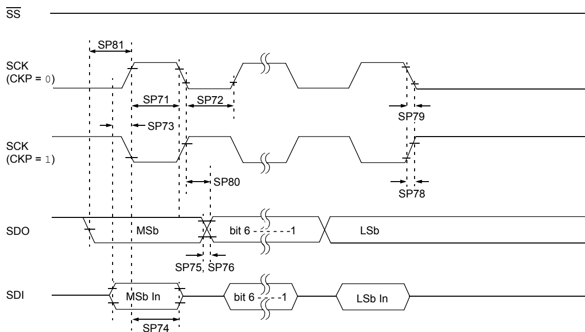
FIGURE 30-17: SPI MASTER MODE TIMING (CKE = 1, SMP = 1)
