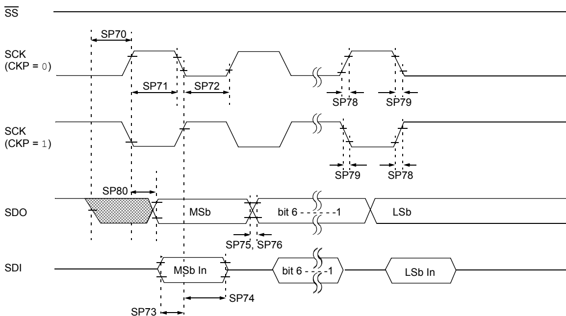
FIGURE 30-16: SPI MASTER MODE TIMING (CKE = 0, SMP = 0)
