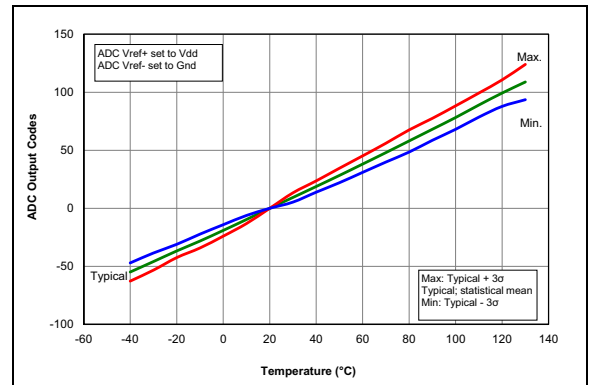
FIGURE 31-106: Temp. Indicator Slope Normalized to 20^\circ C , Low Range, V_{DD} = 3.0V , PIC16LF1782/3 Only.
