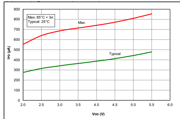
FIGURE 31-46: I_{PD} , Op Amp, High GBWP Mode ( OPA_{xpSP} = 1 ), PIC16F1782/3 Only.
