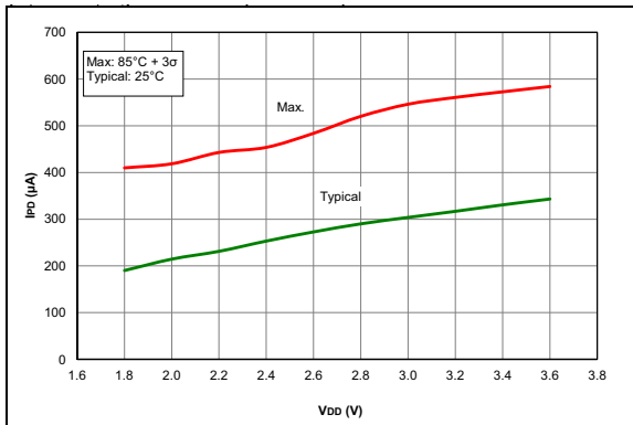
FIGURE 31-45: I_{PD} , Op Amp, High GBWP Mode ( OPA_{xpSP} = 1 ), PIC16LF1782/3 Only.
