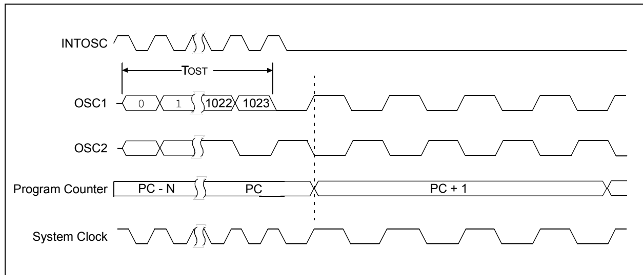
FIGURE 6-8: TWO-SPEED START-UP
