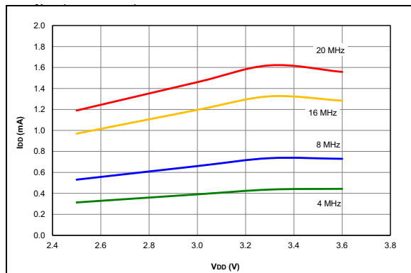
FIGURE 31-27: I_{DD} Typical, HS Oscillator, 25^\circ\text{C} , PIC16LF1782/3 Only.
