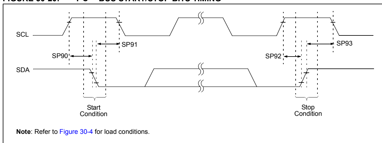
FIGURE 30-20: I 2 C™ BUS START/STOP BITS TIMING
