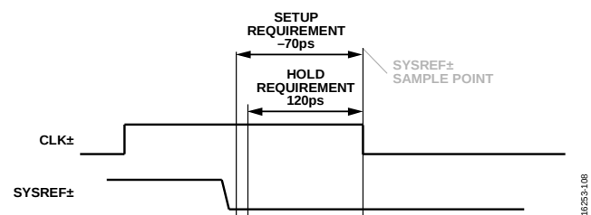
Figure 109. SYSREF± High to Low Transition Using Falling Edge Clock Capture (Register 0x0120, Bit 4 = 1'b1 and Register 0x0120, Bit 3 = 1'b1)
