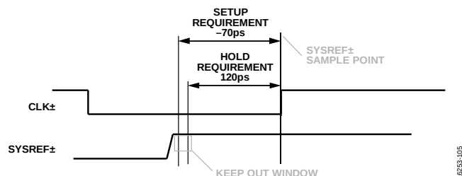
Figure 106. SYSREF± Setup and Hold Time Requirements; SYSREF± Low to High Transition Using the Rising Edge Clock (Default)
