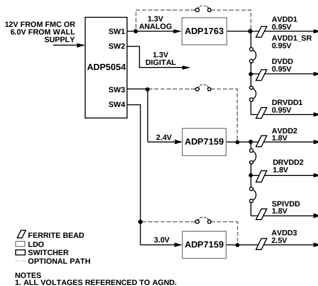
Figure 116. Simplified Power Solution for the AD9697
