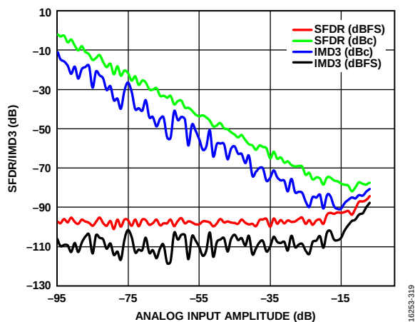
Figure 20. SFDR/IMD3 vs. Analog Input Amplitude, f_{IN} = 172.3 MHz
