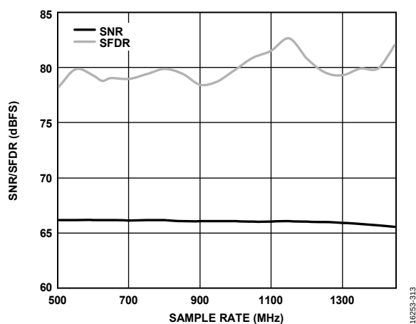
Figure 14. SNR/SFDR vs. Sample Rate, f_{IN} = 172.3\text{ MHz}
