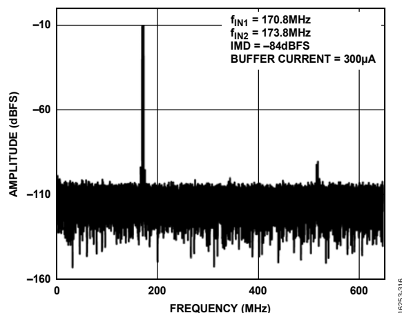
Figure 17. Two-Tone FFT; f_{IN1} = 170.8\text{ MHz} , f_{IN2} = 173.8\text{ MHz}
