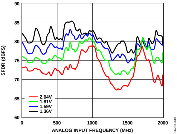
Figure 31. SFDR vs. Analog Input Frequency with Different Analog Input Full-Scale Values
