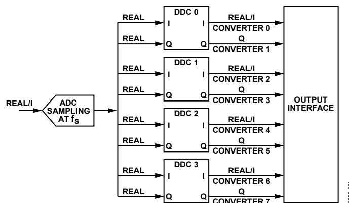
Figure 65. DDCs and Virtual Converter Mapping
