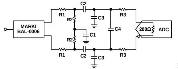
NOTES 1. SEE TABLE 9 FOR COMPONENT VALUES
