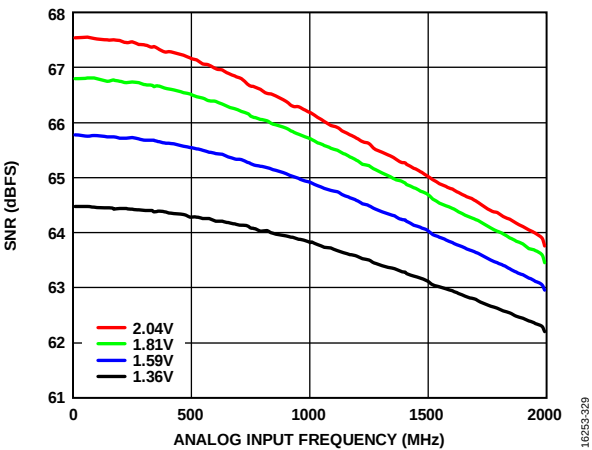
Figure 30. SNR vs. Analog Input Frequency with Different Analog Input Full-Scale Values
