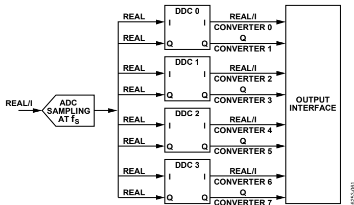
Figure 65. DDCs and Virtual Converter Mapping
