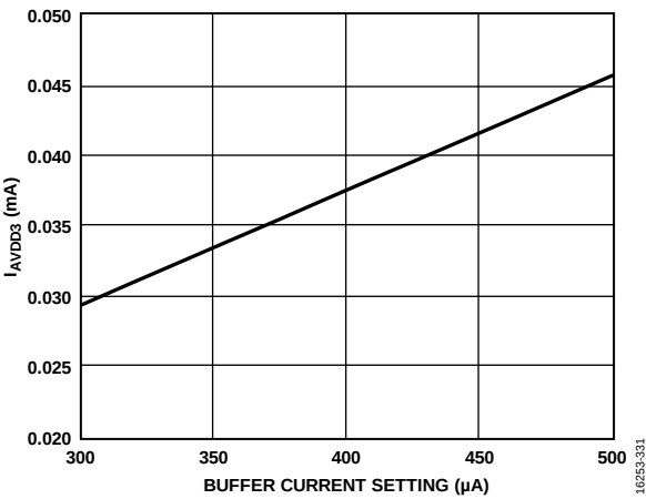
Figure 32. I_{AVDD3} vs. Buffer Current Setting (Buffer Control 1 Setting in Register 0x1A4C)
