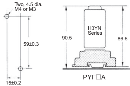
Mounting Holes
