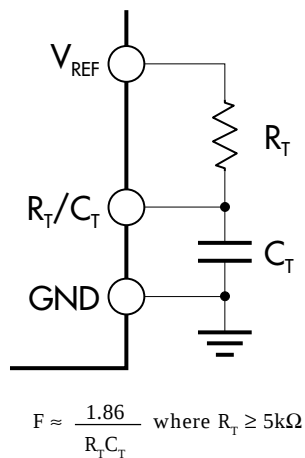
FIGURE 12 — OSCILLATOR TIMING CIRCUIT
