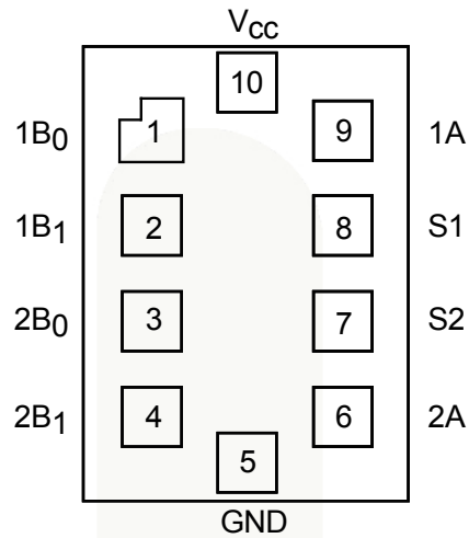
Figure 2. 10-Lead MicroPak™ (Top-Through View)
