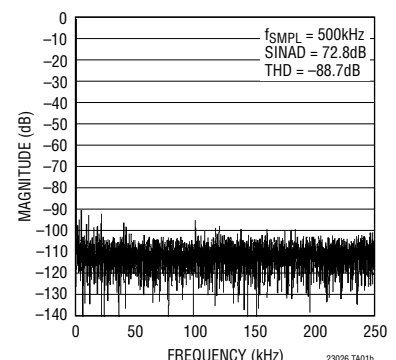
8192 Point FFT, f IN = 1kHz (LTC2306)
