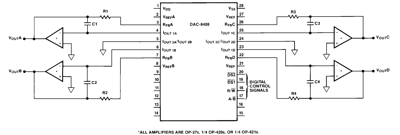
Figure 6. Quad DAC Unipolar Operation (2-Quadrant Multiplication)
