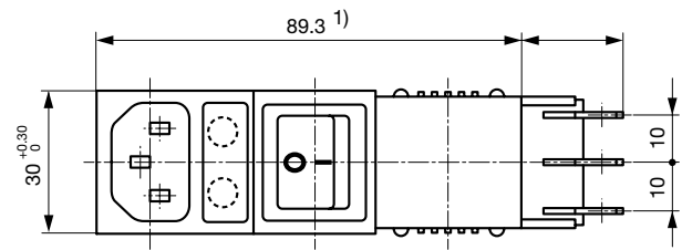
Variants 5424.XX5X.XXX Mounting hole: 87.9 +0.2 \times 27.6 +0.2 A: Quick-connect terminal 6.3x0.8 mm: 22 mm A: Solder terminal 3.5x0.8 mm: 17.5 mm S: Panel thickness
