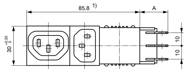
Variants 5421.X05X.XXX Mounting hole: 85.9 +0.2 \times 27.6 +0.2 A: Quick-connect terminal 6.3x0.8 mm: 22 mm A: Solder terminal 3.5x0.8 mm: 17.5 mm S: Panel thickness
