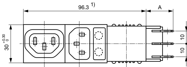
Variants 5423.XX5X.XXX Mounting hole: 96.4 +0.2 \times 27.6 +0.2 A: Quick-connect terminal 6.3x0.8 mm: 22 mm A: Solder terminal 3.5x0.8 mm: 17.5 mm S: Panel thickness
