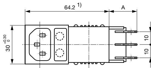
Variants 5411.XX5X.XXX Mounting hole: 63 +0.2 \times 27.6 +0.2 A: Quick-connect terminal 6.3x0.8 mm: 22 mm A: Solder terminal 3.5x0.8 mm: 17.5 mm S: Panel thickness
