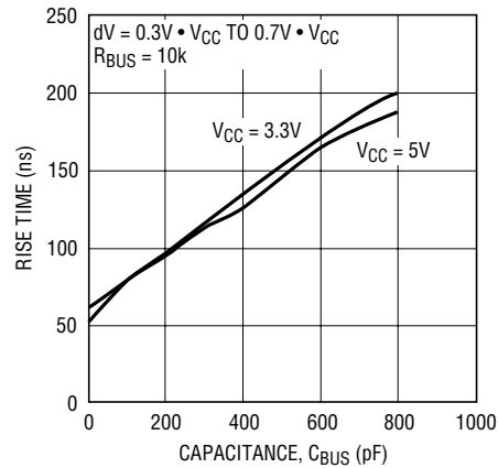
Rise Time vs C_{BUS} vs V_{CC}
