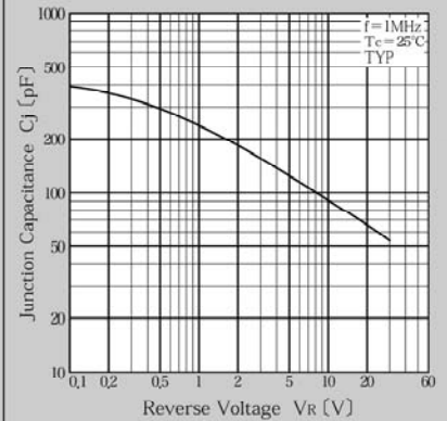
Junction Capacitance
