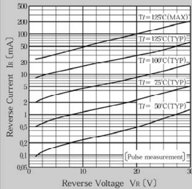
Reverse Current
