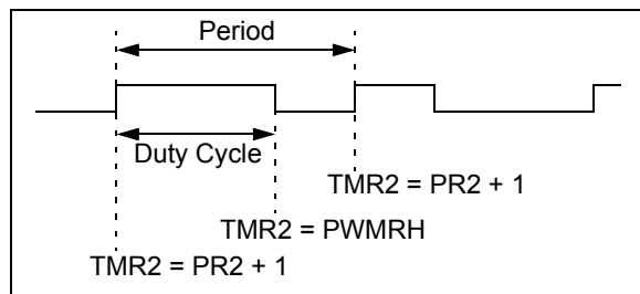
FIGURE 25-2: PWM OUTPUT
