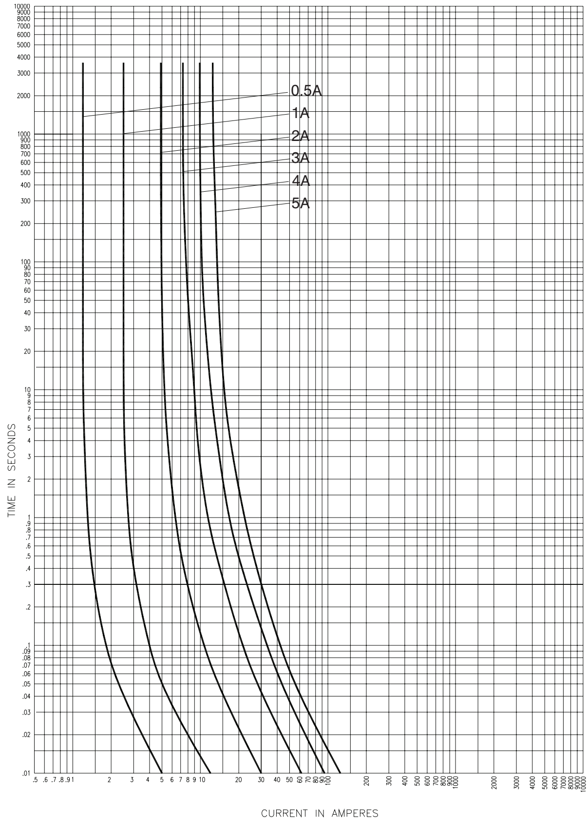
5.5kV time-current curves — total clearing for 5NCLPT_
