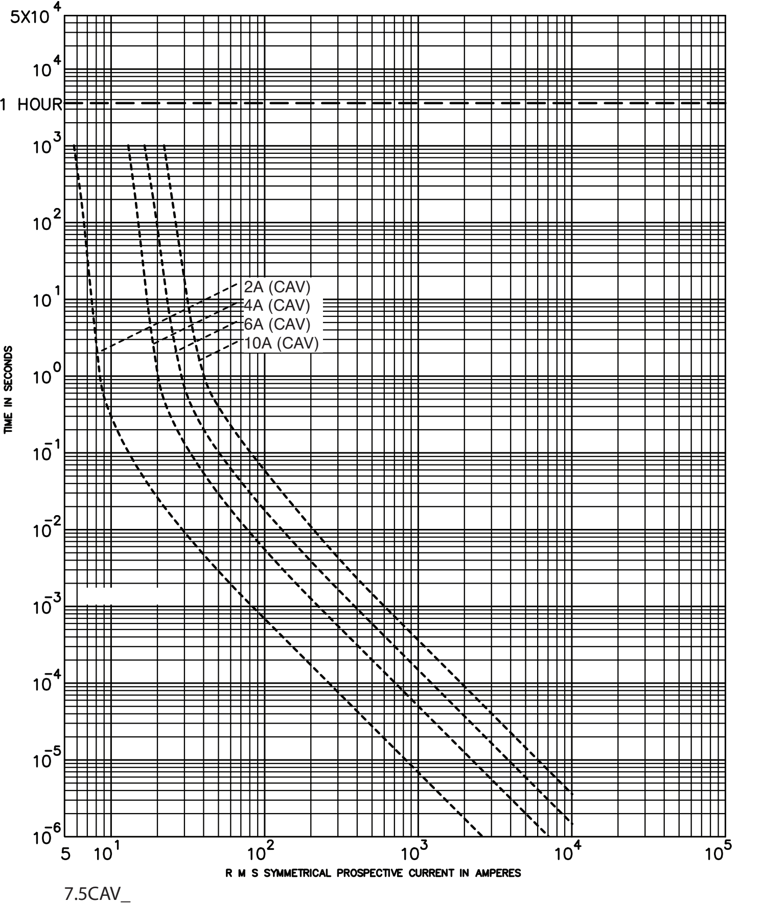
17.5kV time-current curves — minimum melting for 17.5CAV_
