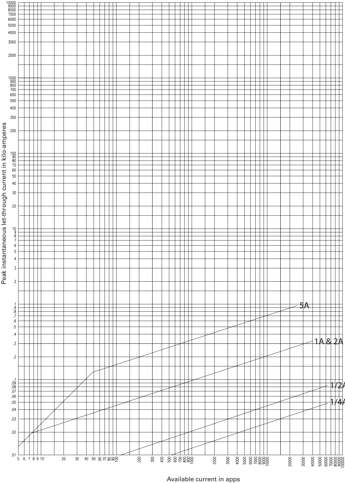
2.47kV peak let-through curves for 2NCLPT_E
