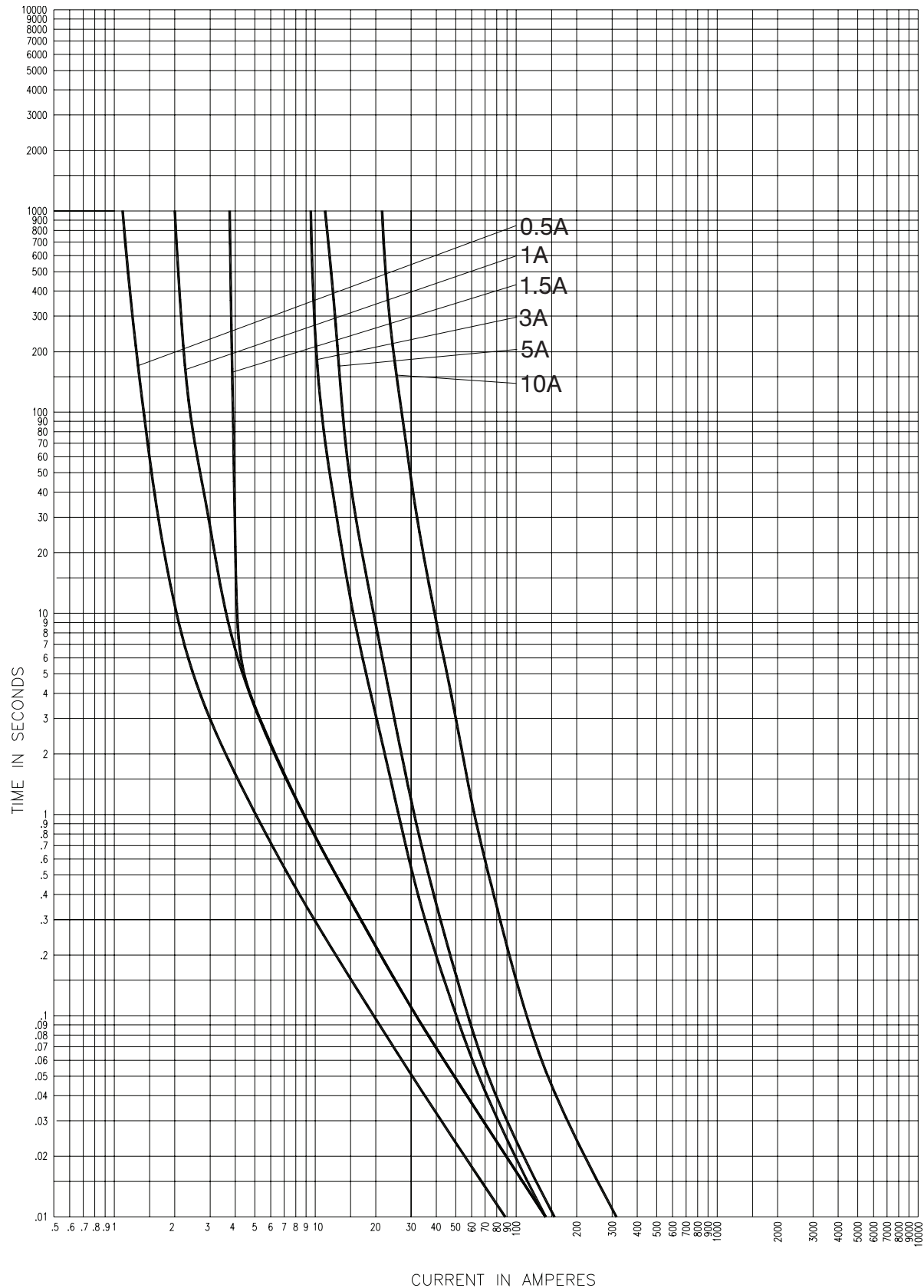
15.5kV time-current curves — minimum melting for 15CLPT_
