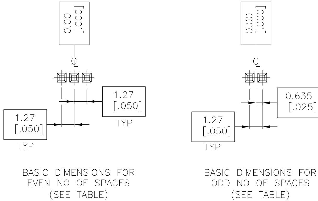
DETAIL R
