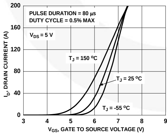
Figure 54. Transfer Characteristics
