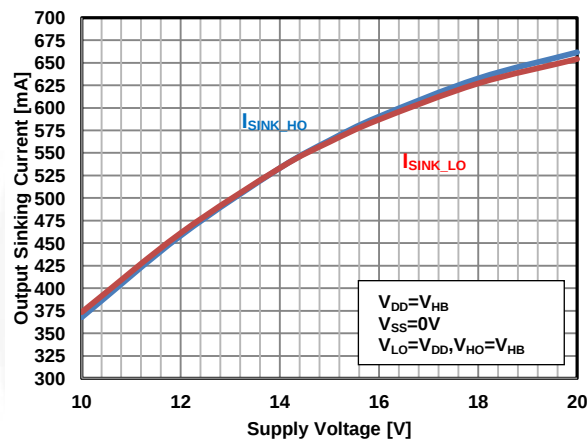
Figure 23. Output Sinking Current vs. Supply Voltage ( V_{DD} )
