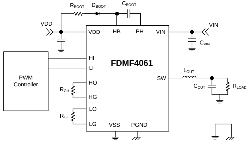
Figure 6. Buck Converter
