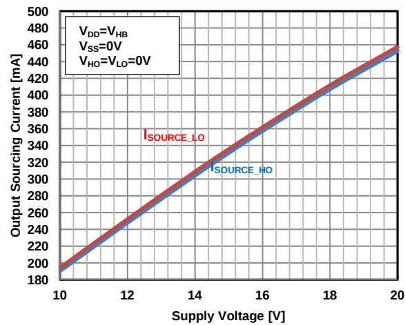
Figure 21. Output Sourcing Current vs. Supply Voltage ( V_{DD} )
