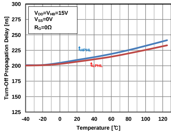
Figure 16. Turn-Off Propagation Delay vs. Temp.
