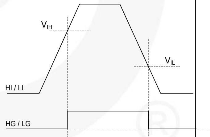
Figure 63. PWM threshold definitions
