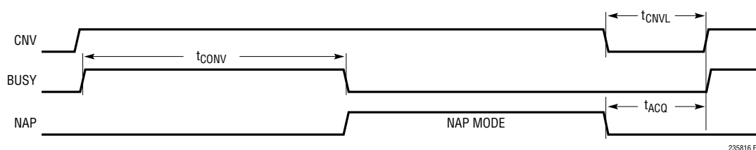
Figure 13. Nap Mode Timing for the LTC2358-16
