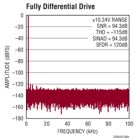
Figure 6c. IN^+/IN^- = -1\text{dBFS} 2kHz Fully Differential Sine, V_{\text{CM}} = 0\text{V} , 32k Point FFT, f_{\text{SAMPL}} = 200\text{kpsps} . Circuit Shown in Figure 6a
