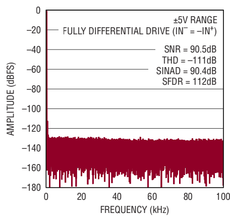
Figure 7c. IN + /IN - = 450mV 200Hz Fully Differential Sine, 0V ≤ V CM ≤ 24V, 32k Point FFT, f SMPL = 200ksps. Circuit Shown in Figure 7a
