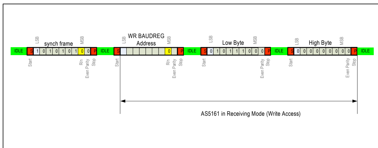
Figure 31: Manual Baud-Rate Setting
