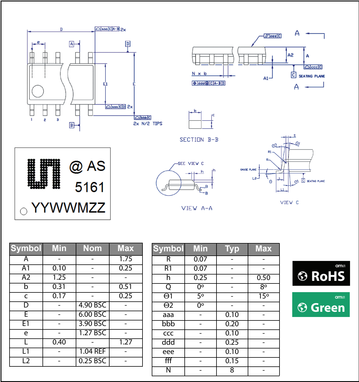
Figure 38: Package Drawings and Dimensions
