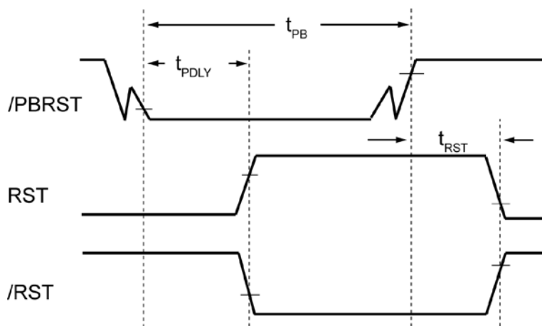
Figure 3. Pushbutton Reset
