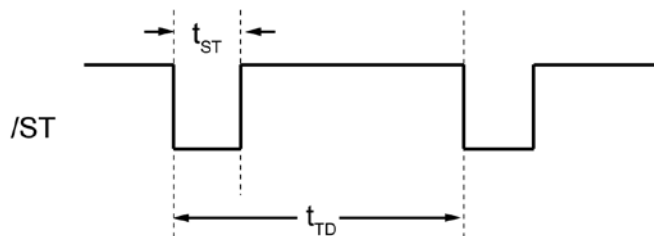
Figure 2. Watchdog Input
