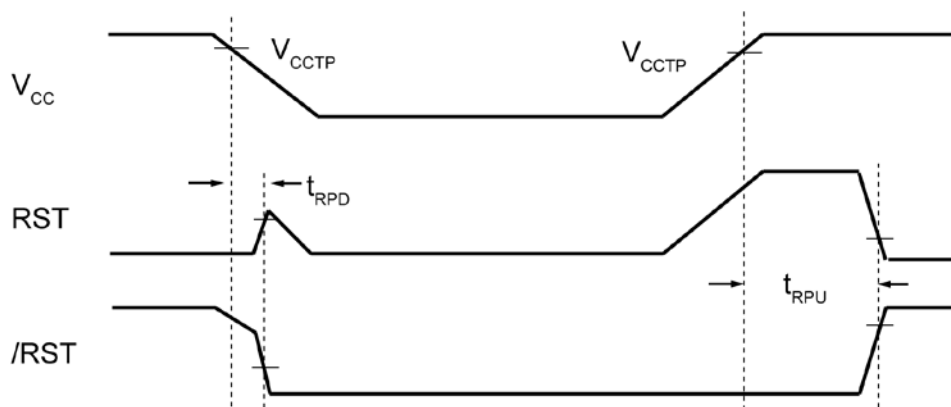
Figure 1. Power-Up/Power-Down Sequence
